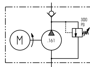
HYDRAULIC SCHEMATIC
